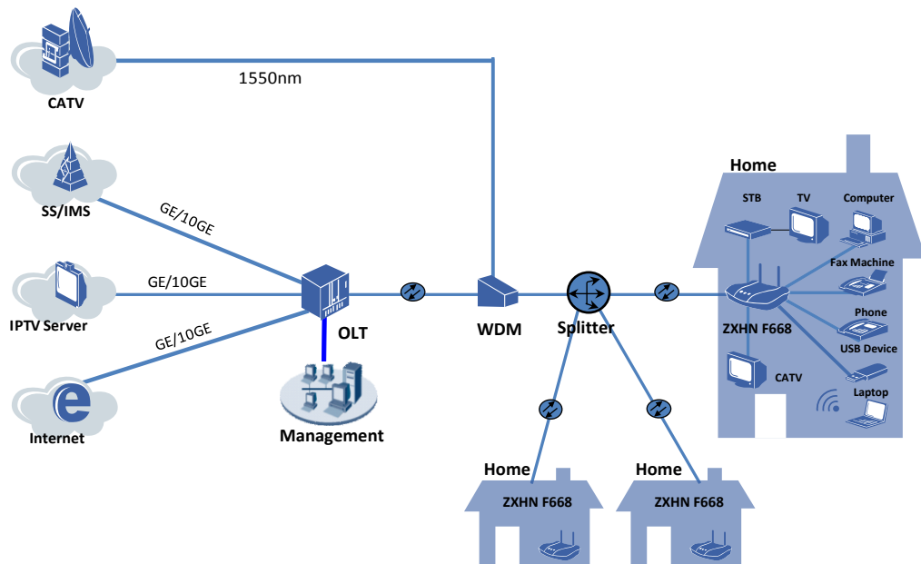
Figure 1-2 Application Scenario of the ZXHN F668
